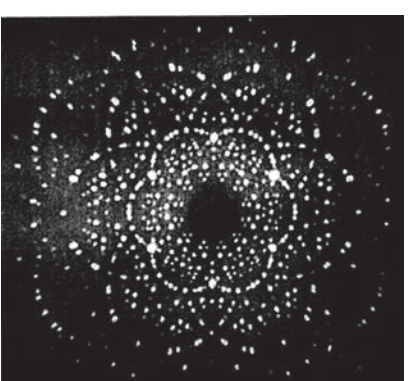
Fig. 6-28. Atomic pattern of a beryl crystal.
