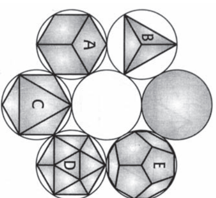
Fig. 6-15. The five Platonic solids.
