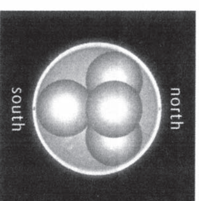
Fig. 7-12. The first four cells form a tetrahedron.
