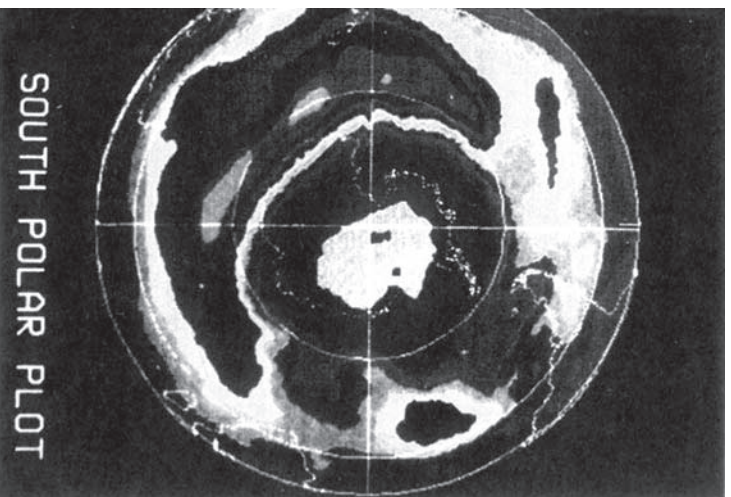
Fig. 3-4. Ozone hole above the South Pole.
