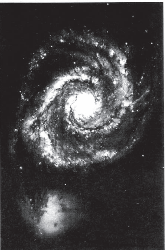
Fig. 8-30. Swirling galaxy.
