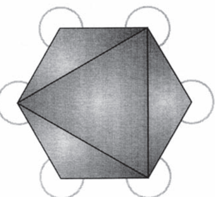
Fig. 6-18a. Solid larger octahedron.
