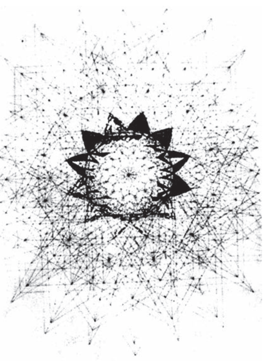
Fig. 6-4. Twice-ratcheted Genesis pattern with all possible connected lines.
