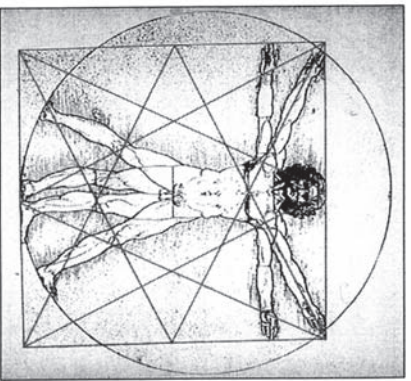
Fig. 7-41. Diagonal lines made by connecting corner to the center of the opposite side of the square.
