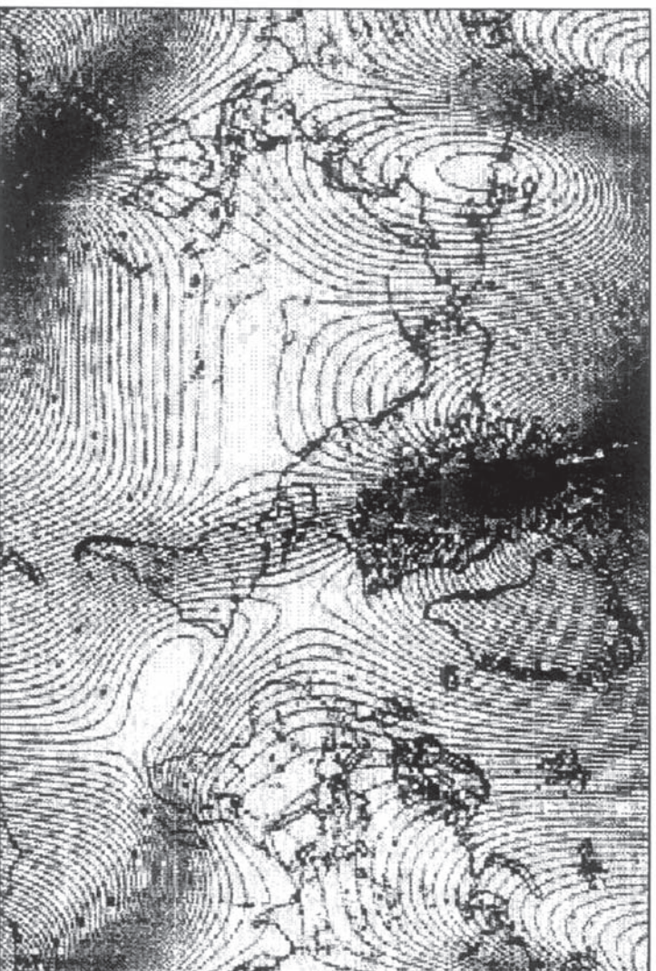
Fig. 2-44. Sample of complex model of Earth's main magnetic field, generated by the USGS for the year 1995.
