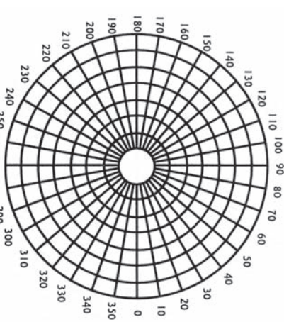
Fig. 8-22. Polar graph.
