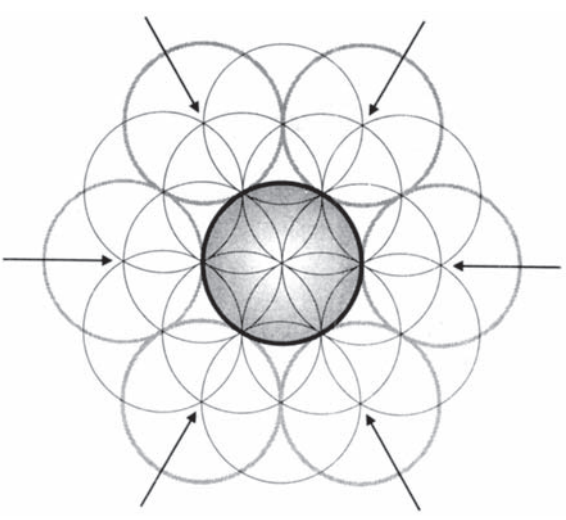
Fig. 6-9. The third rotation.
