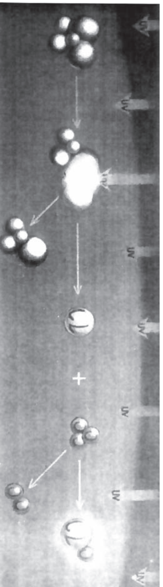
Fig. 3-5. Ozone reaction in molecules.
