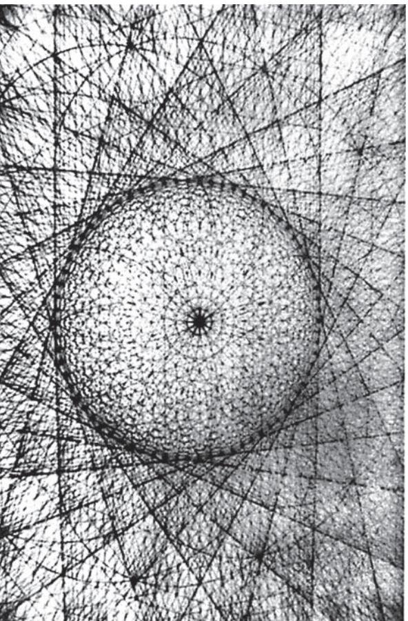
Fig. 6-2. Genesis pattern ratcheted once.
