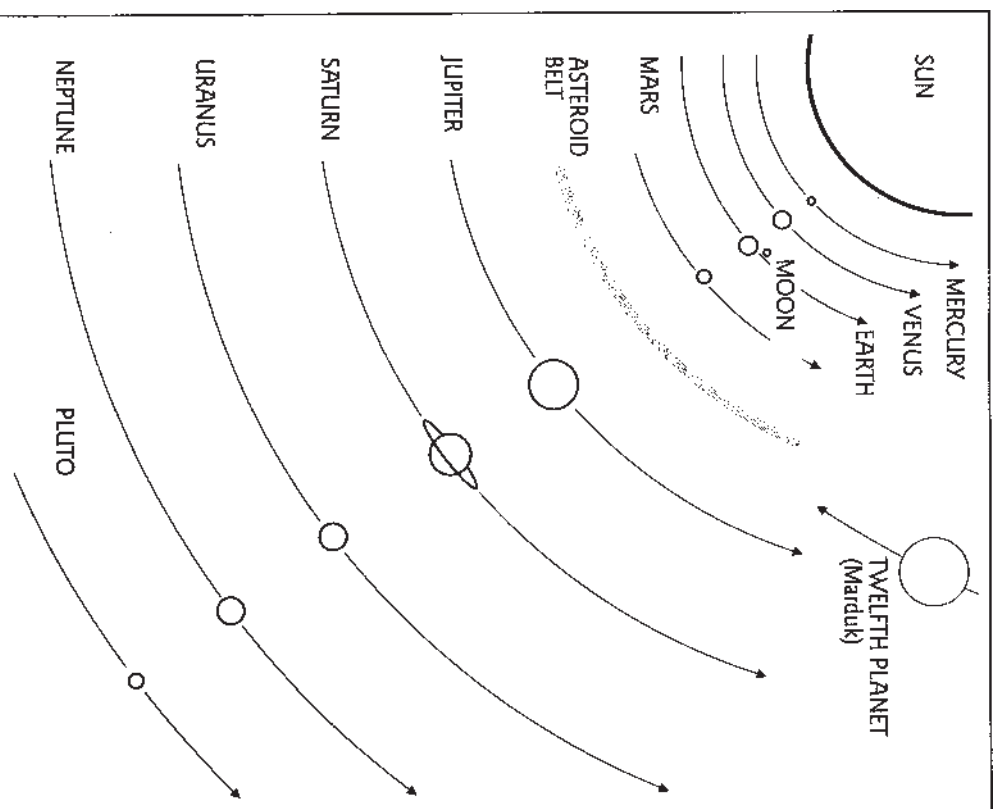
Fig. 3-8. Solar system including Marduk/Nibiru and the remains of Tiamat (asteroid belt and Earth)
