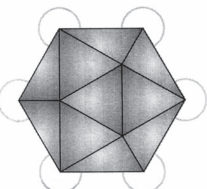
Fig. 6-19a. Solid larger icosahedron.
